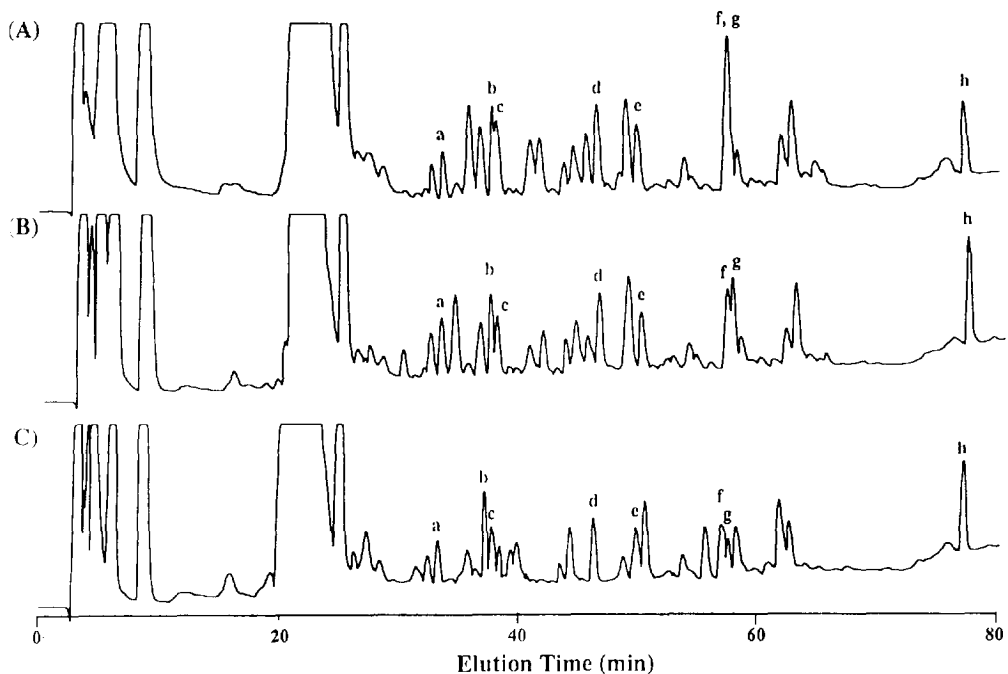
Fig. 4. Resolution of the alkylated trypsin digests of isotoxins. The alkylated derivatives of (A) P8, (B) P9 and (C) P11 were resolved by HPLC on a reversed-phase C 18 column, which was washed consecutively with 0.1% trifluoroacetic acid (TFA) for 5 min, a linear gradient of 0-30% acetonitrile in 0.1% TFA for 60 min, a linear gradient of 30-60% acetonitrile in 0.1% TFA for 10 min and 60% acetonitrile in 0.1% TFA for 5 min. The flow-rate was 1 ml/min and the effluent was monitored at 214 nm. Peptides a-h of each protein sample were pooled for automated Edman degradation.
